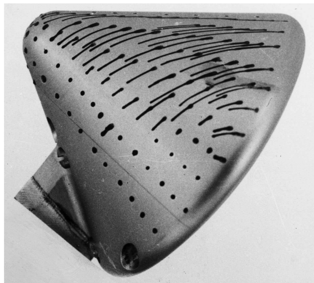
Fig. 36 Photograph and sketch of oil-flow pattern on Apollo at 35 deg AOA and Mach 8, showing lee separation. Flow from right to left. From Fig. 9 in [75].
